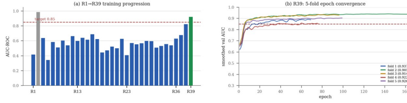
Fig. 2. (a) Mean/best AUC across all 39 tracked training runs, R39 (749-model corpus) highlighted. (b) R39’s five-fold validation-AUC convergence, final test AUC per fold in the legend.
